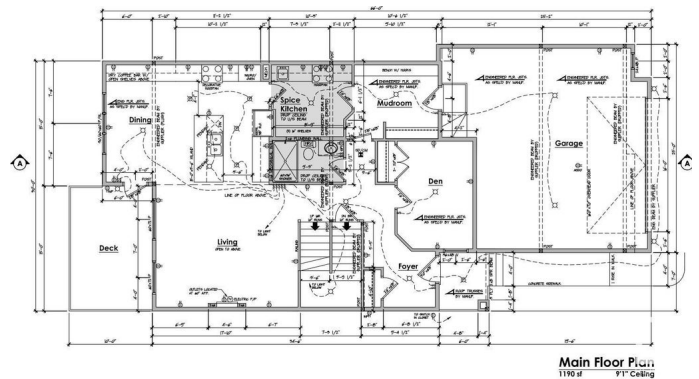
Main Floor Plan 1190 sq ft 9' Ceiling
